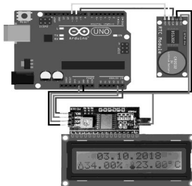
Pic. 6. Schematic diagram of the monitoring subsystem
