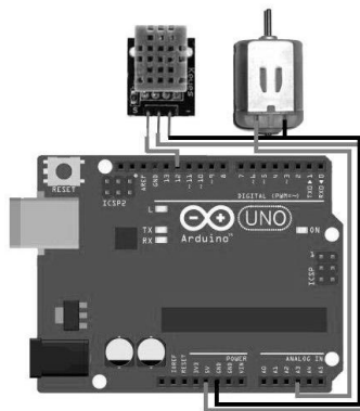
Pic. 5. The scheme of the climate control subsystem
