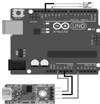
Pic. 4. Scheme of the lighting control subsystem
