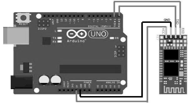
Pic. 2. Bluetooth HC-06 connection scheme
