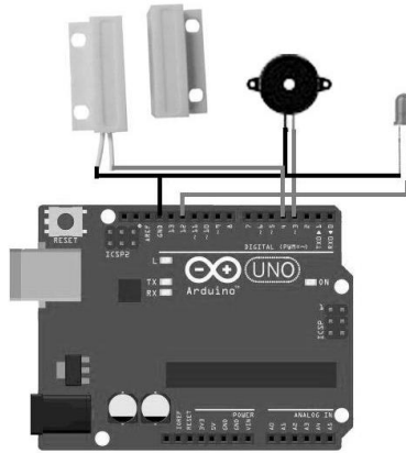
Pic. 3. Scheme of the alarm system
